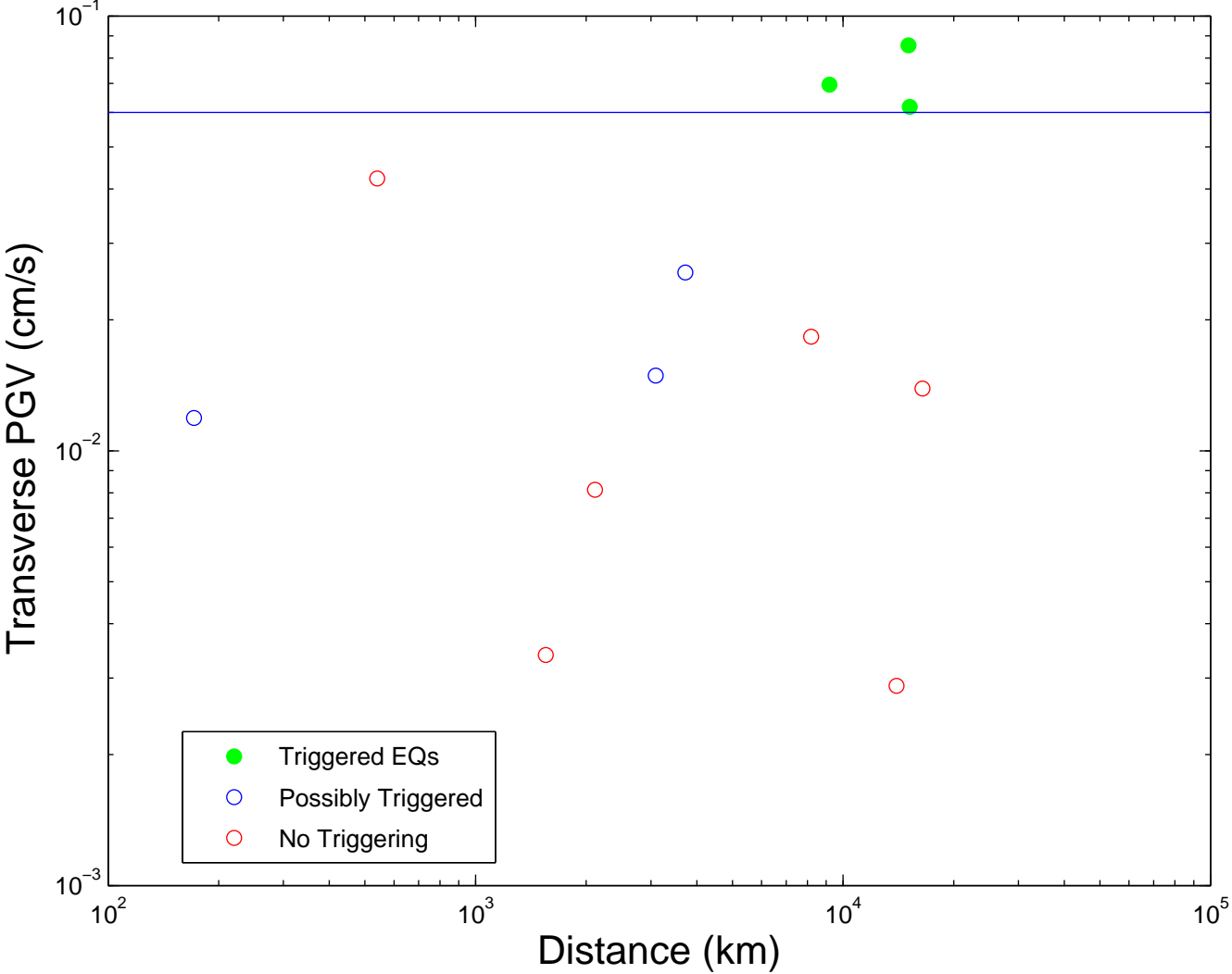
Transverse PGV vs. Dist – Southern Chile
