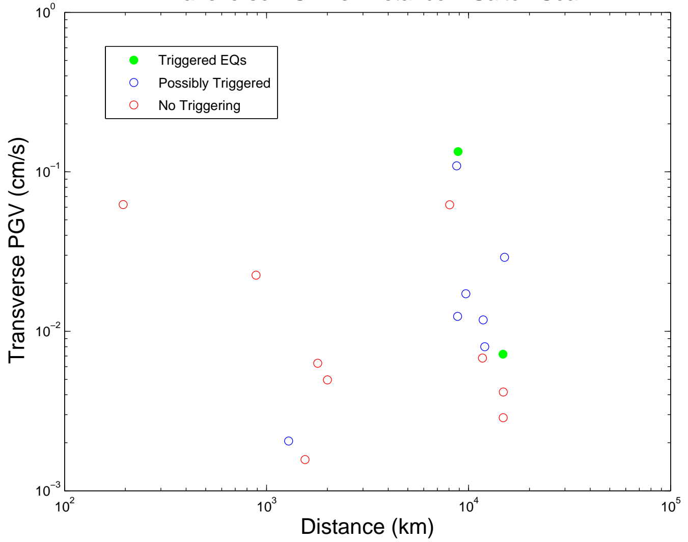
Transverse PGV vs. Distance – Salton Sea
