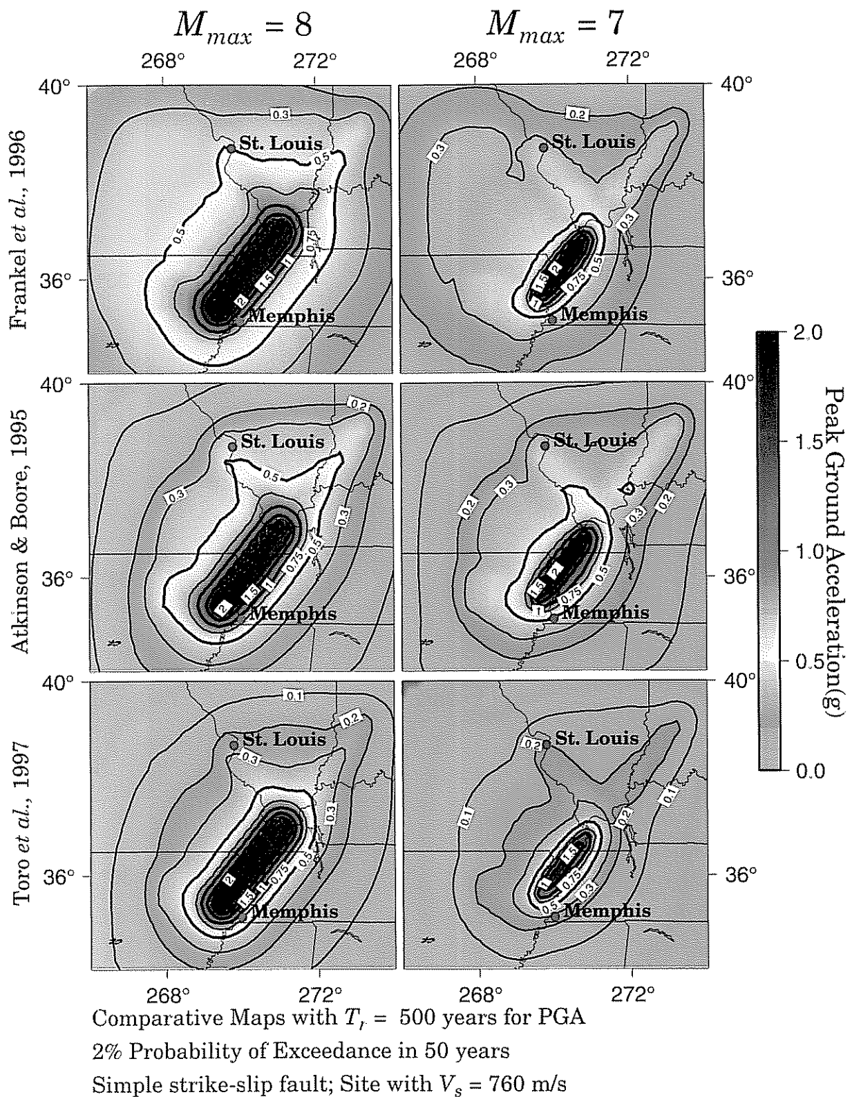
▲ Figure 4. Comparison of the predicted hazard (PGA for 2% probability in 50 years) for “firm rock” sites, corresponding to different maximum magnitude and ground motion relations, for T_r of 500 yr. The values are higher and vary for different M_{max} and ground-motion relations in ways similar to those for T_r of 1,000 yr (Figure 3).
