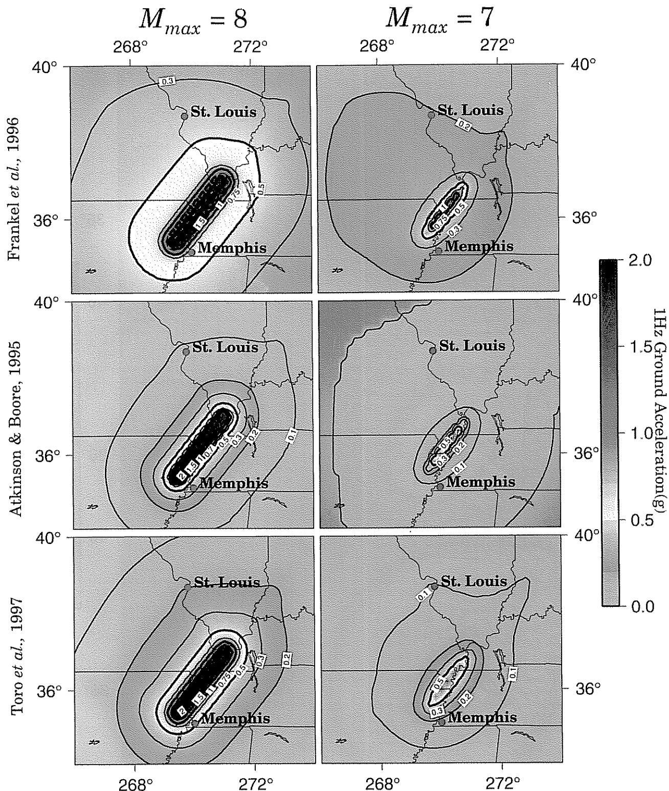
Comparative Maps with T_r = 500 years for 1 Hz 2% Probability of Exceedance in 50 years Simple strike-slip fault; Site with V_s = 760 m/s
