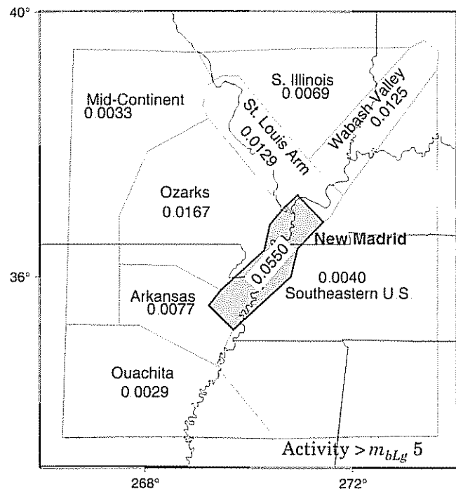
▲ Figure 2. Area source geometry used in hazards modeling. Areas represent differences in underlying geology, and their seismicity is described by the annual activity rates of earthquakes shown.
