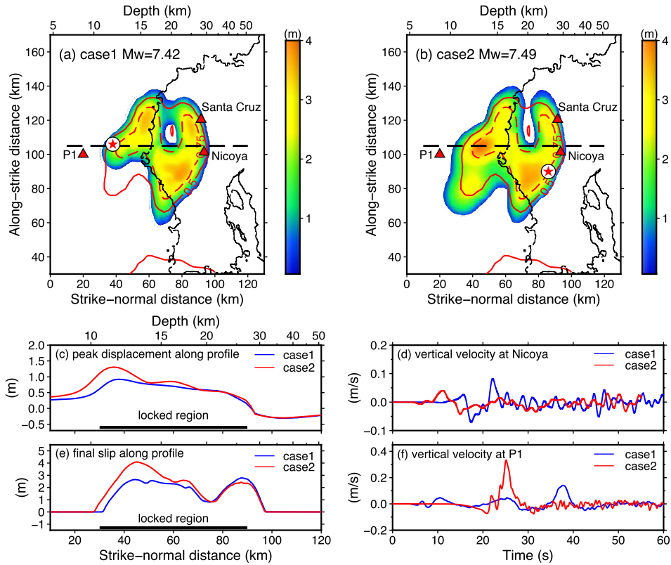
Fig. 5. Final slip distribution of rupture scenarios nucleated at two different locations, offshore (a) and inland (b), using the Feng locking model (contours) with nucleation sizes of 4 km. Dash lines show a profile to compare ground displacements. Triangles denote hypothetical stations, one offshore (P1) and two at towns of Nicoya and Santa Cruz. Peak displacements (c) and final slip distribution (e) along the profile from the two rupture scenarios. Vertical velocities recorded at Nicoya (d) and P1 (f) from the two scenarios, respectively.
