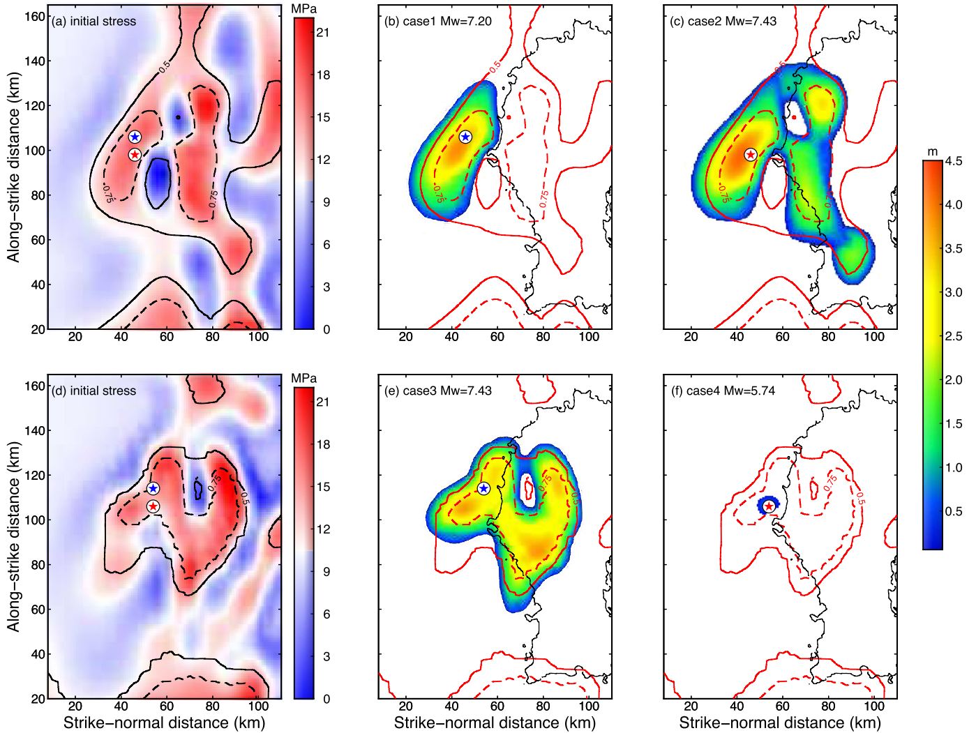
Fig. 2. (a) Initial stress distribution that is derived from interseismic locking distribution (Xue et al., 2015). Blue and red stars denote two nucleation zones at the same depth, having identical initial stresses and sizes (5 km). (b) and (c), Slip distribution of scenario earthquakes that were initiated from the blue (b) and red (c) stars. Solid and dashed lines show the locking model. (d), (e), and (f) are same to (a), (b), and (c) panels, respectively, except these are for the Feng locking model (Feng et al., 2012).
