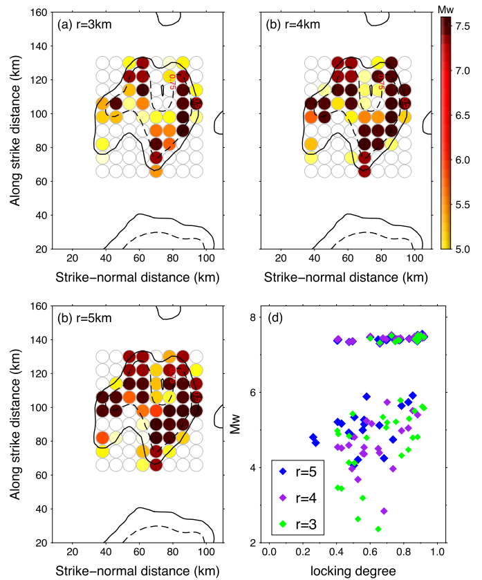
Fig. 4. Same with Fig. 3, except for the Feng locking model.
